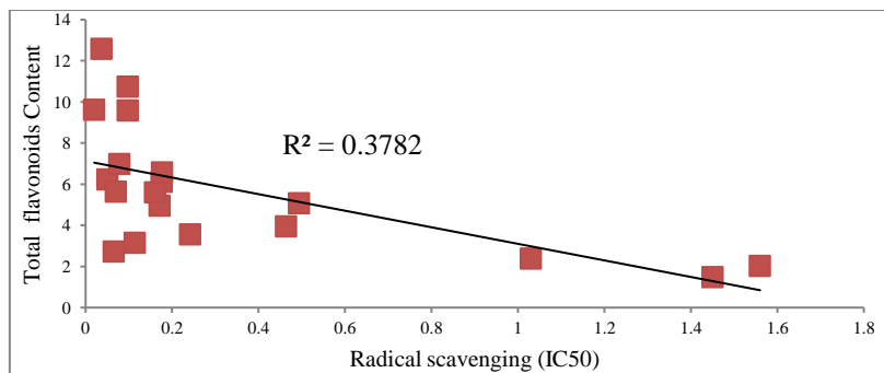
Figure 2: Correlation of flavonoid content and IC_{50} radical scavenging
